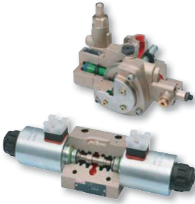
Cutaway Models
